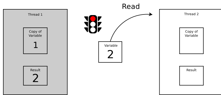
Figure 124: How mutex works (5/8)
